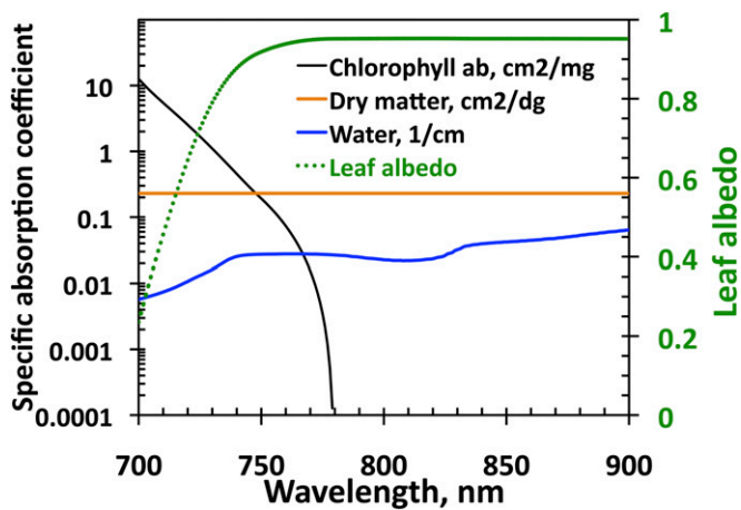
Fig. 4. Absorption spectra of chlorophyll ab (in \text{cm}^2/\text{mg} ), dry matter (in \text{cm}^2/\text{dg} ), and water (in \text{cm}^{-1} ) (vertical axis on the left side) and spectrum of leaf albedo (vertical axis on the right side) from the PROSPECT-5 model (45). In these units values of typical concentrations of these absorbing pigments are on the order of 0.05. Impact of water absorption can be neglected.
